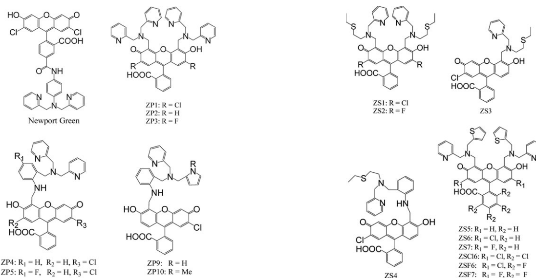
Scheme 7 Structures of the Zinspy (ZS) family sensors.
